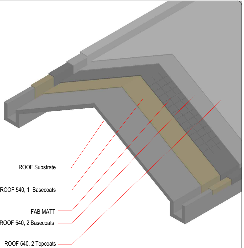
Title: ROOF 540 Low Slope Roof Coating Detail Version:01 Revised Date: 1/8/12 Date: 10/10/10
