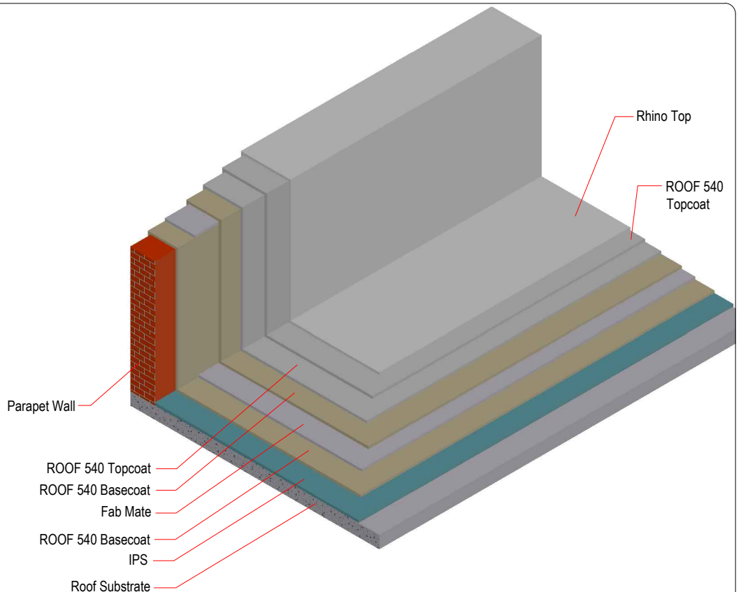
Title: ROOF 540 Parapet Wall Coating Details Version: 01 Revised Date: 01/08/12 Date:
